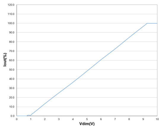
Dimming Curve:
