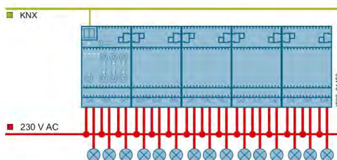
Diagram of 15-fold switching actuator
